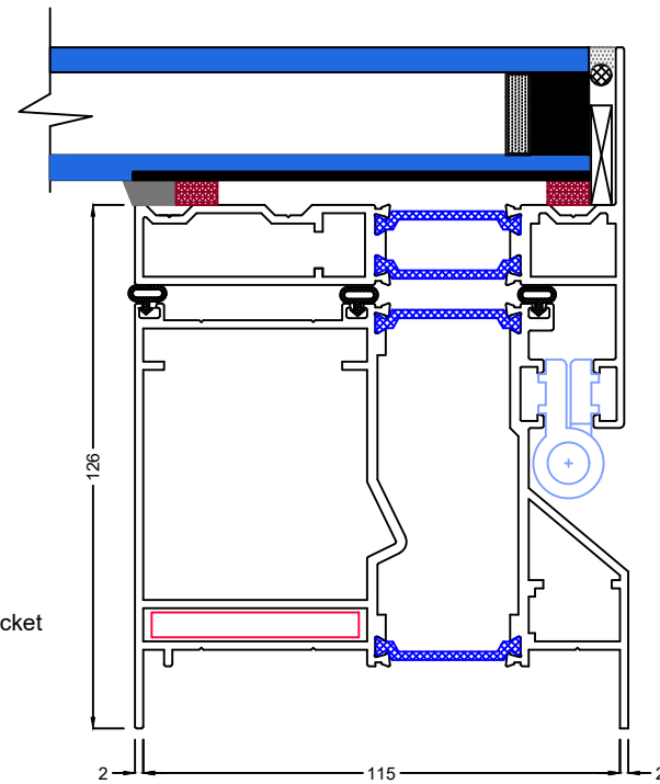
B Section thru Hinge side. (Closed position)
