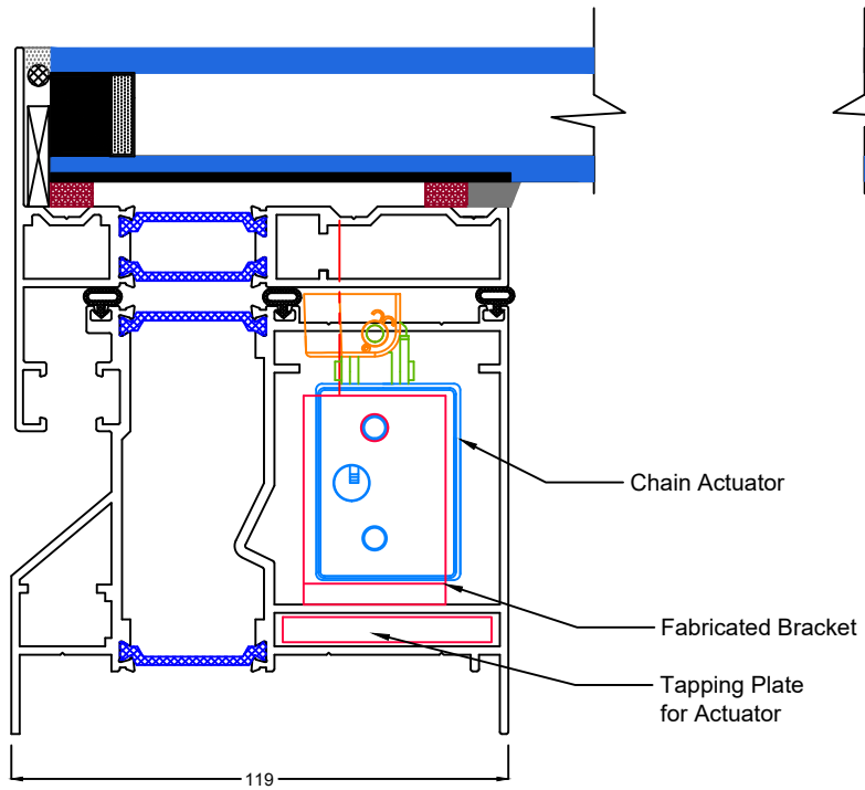
A Section thru Actuator side. (Closed position)
